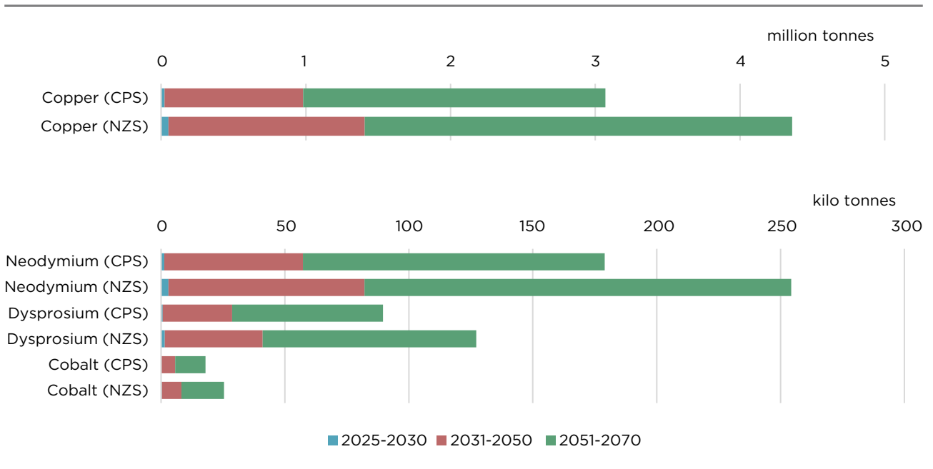
Figure 2.7: EV Motors - Embedded Mineral Requirements
