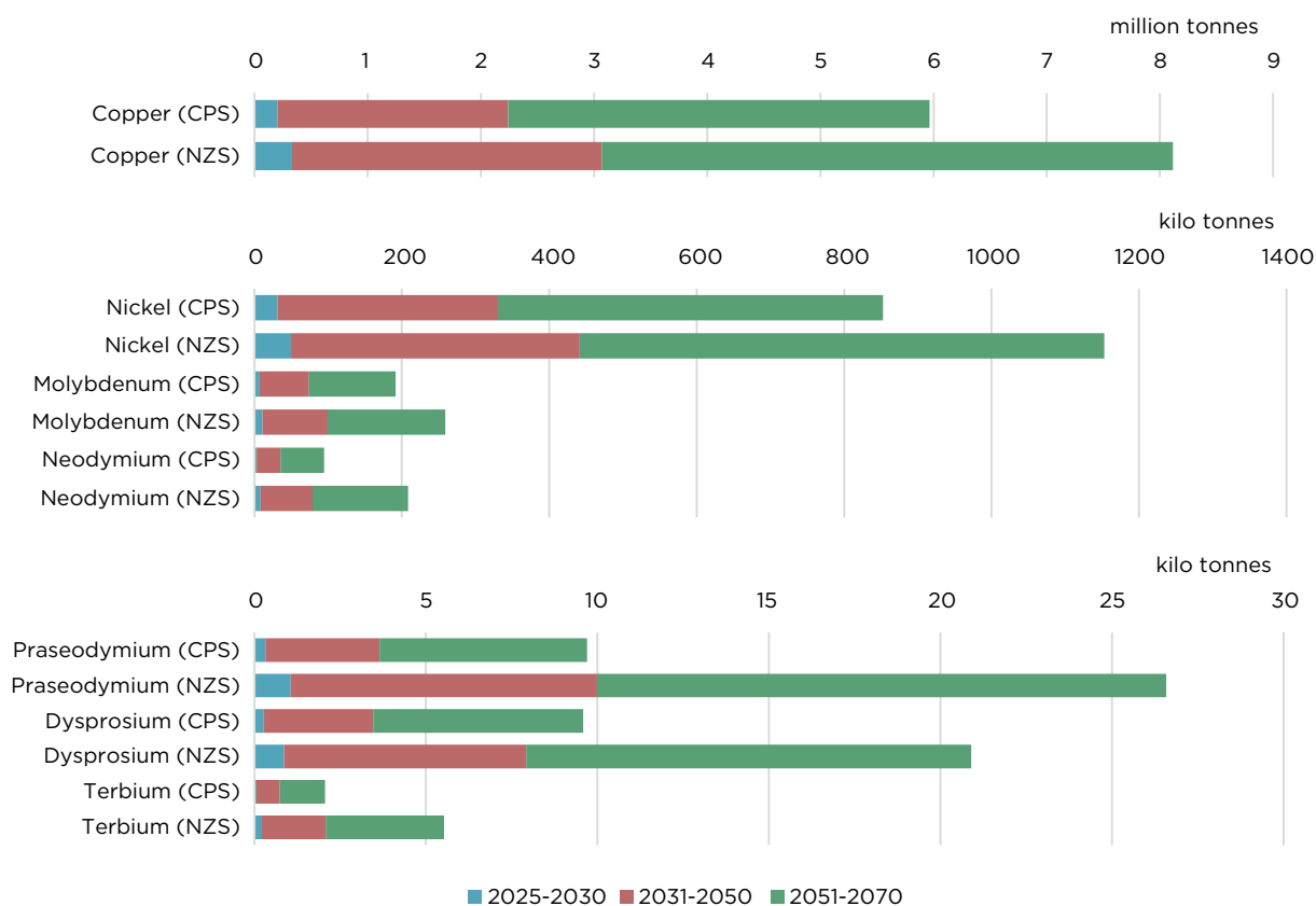
Figure 2.3: Onshore Wind - Embedded Mineral Requirements under Current Policy Scenario (CPS) and Net Zero Scenario (NZS)
