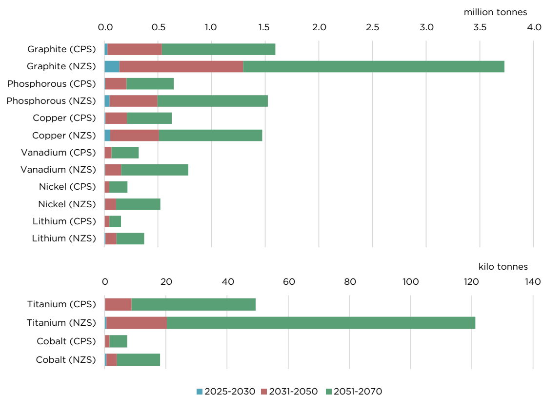
Figure 2.5: Stationary Battery Energy Storage - Embedded Mineral Requirements under Current Policy Scenario (CPS) and Net Zero Scenario (NZZS)
